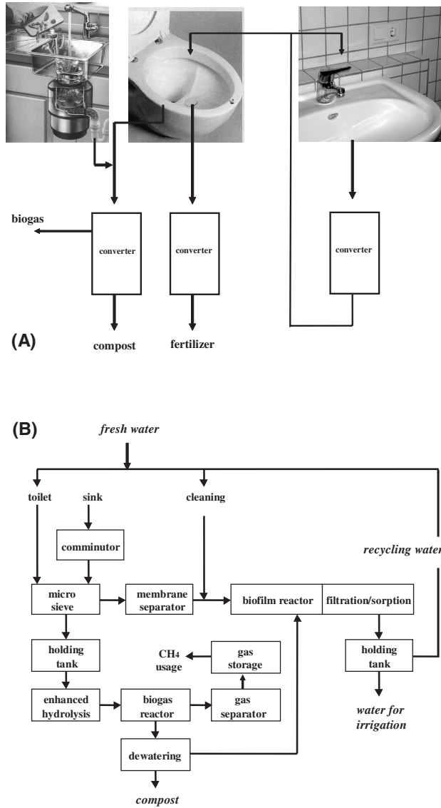
Figure 3 Example of a concept (A), and a flow schematic (B) of a small on-site system to treat separately black, green and gray water
