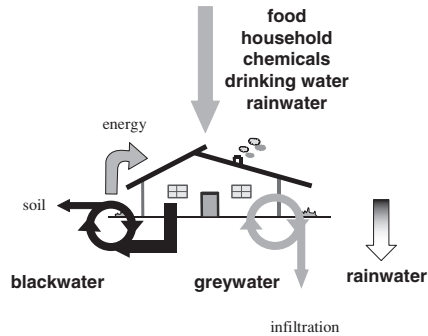
Figure 2 Schematic representation of an on-site water management system based on the concept of source separation, treatment of the individual wastewater fractions, recovery and reuse of valuable materials
